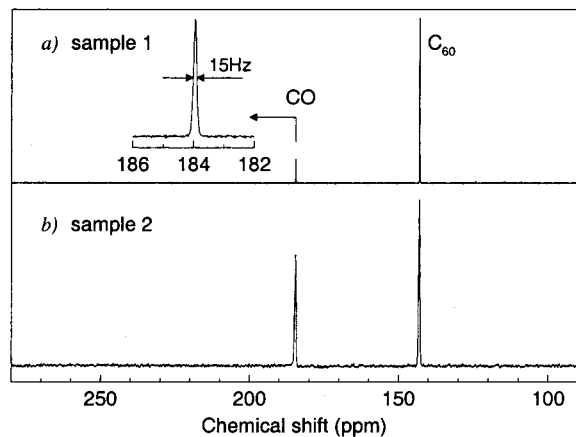
Figure 1. (a) ^{13}\text{C} NMR spectrum of ^{13}\text{CO} -intercalated \text{C}_{60} sample no. 1 measured in the AM500 spectrometer under magic-angle-spinning conditions at room temperature. This spectrum is recorded by summing 30 scans using a relaxation delay of 125 s. The inset shows an expanded view of the observed CO resonance. (b) The same for sample no. 2, but recorded on the DMX300 spectrometer by summing 16 scans with a relaxation delay of 400 s. The chemical shift in both spectra is referenced to tetramethylsilane (TMS).
