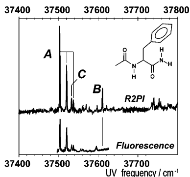
Figure 2. Mass-selective one-color R2PI spectrum (top) and excitation fluorescence spectrum (bottom) of the model peptide N -Ac-Phe-NH 2 in the origin region of the S_1 \leftarrow S_0 transition of the phenyl chromophore. Conformational features are identified and labeled according to the isomers deduced from the resonant ion-dip IR experiments.
