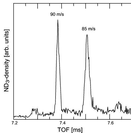
Fig. 9 Density of \text{ND}_3 molecules 36 cm behind the decelerator as a function of time after release of the gas pulse. Two 3D-spatially focused packets of molecules with forward velocities as indicated are observed. The length of each packet is about 2 mm, the separation between the packets is about 11 mm.
