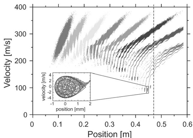
Fig. 2 Numerical simulations of the phase-space distribution of an ensemble of \text{ND}_3 molecules passing through the decelerator for eight different times. In the inset, the phase-space distribution of a decelerated packet is shown in the moving frame of the synchronous molecule. The dashed vertical line indicates the position at which the TOF measurements shown in Fig. 6 are taken.
