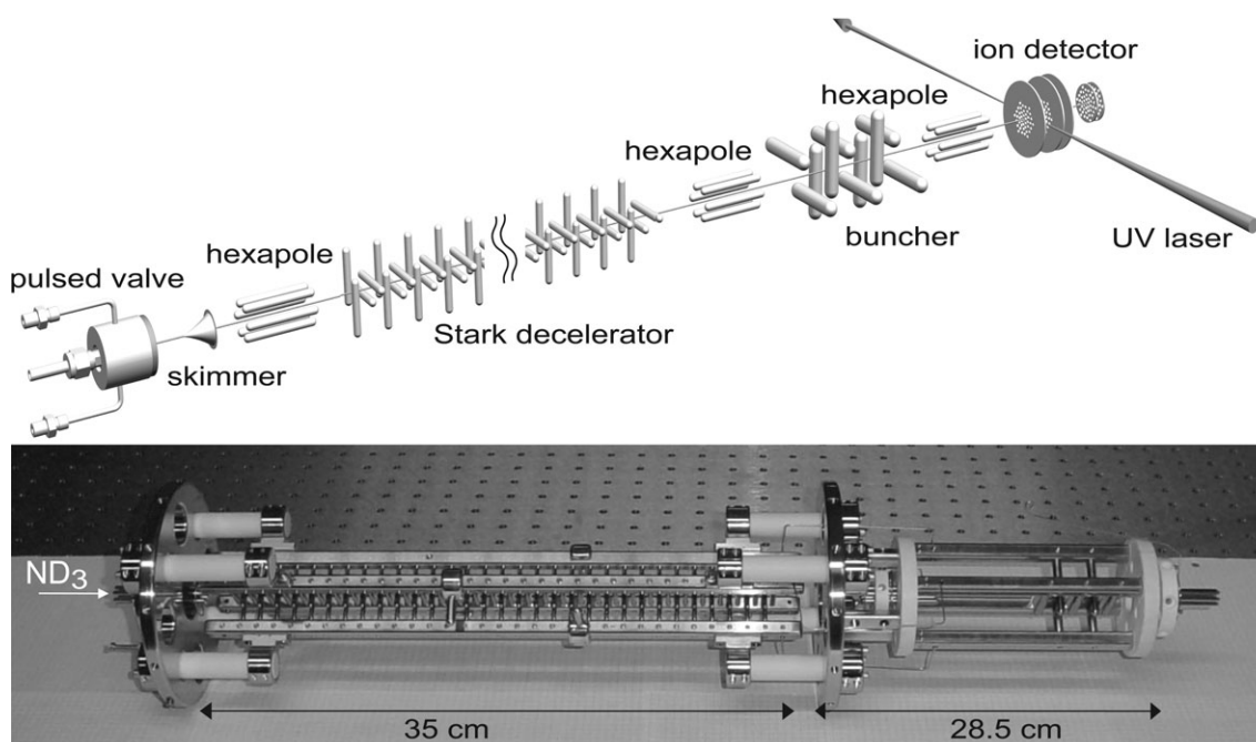
Fig. 5 Scheme of the molecular beam machine. \text{ND}_3 molecules seeded in Xe expand through a nozzle at a 10 Hz rate. After passing through a skimmer, molecules in the low-field seeking |J,KM\rangle = |1,-1\rangle level are focused with a hexapole into the Stark decelerator. The decelerated molecules pass through a hexapole–buncher–hexapole combination prior to entering the detection region. There, the density of the ammonia molecules is state-selectively detected using a UV-laser ionization scheme (2 + 1 REMPI). Below, a photo is shown of the main components: (from left to right) hexapole, decelerator, hexapole, buncher, hexapole.
