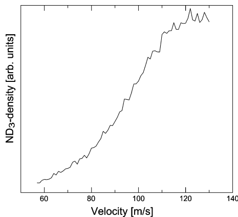
Fig. 8 The density of \text{ND}_3 molecules 36 cm behind the decelerator as a function of velocity. For each velocity, the molecules are 3D-spatially focused into the interaction region.
