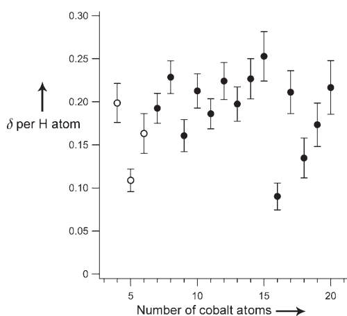
Figure 2. Average \delta values for [\text{Co}_n]^+ clusters ( n=4\text{--}20 ). Open symbols indicate values obtained from a fit of the data to Equation (3); solid symbols indicate that only values of the monocarbonyl and hydrogen saturated complexes have been used.
