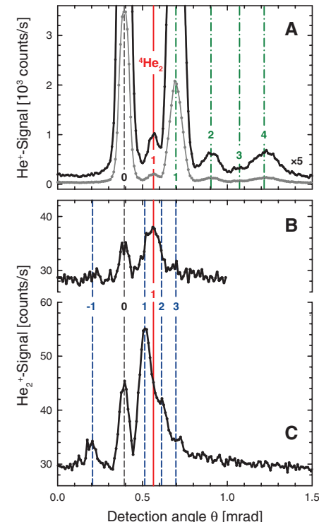
Fig. 2. Diffraction patterns of helium beams for two different stagnation pressures and measured with two different mass channels of the detector. (A) The 4-amu mass channel, P_0 = 1 bar. (The dark trace represents a fivefold magnification of the intensity.) (B) The 8-amu mass channel, P_0 = 1 bar. (C) The 8-amu mass channel, P_0 = 2 bar. At 4 amu (A), atoms and, due to fragmentation in the detector, also clusters can be detected, whereas at 8 amu (B and C) the atomic component of the beam is absent. The calculated diffraction angles of He, He 2 , and He 3 are indicated by green dash-dotted, red solid, and blue dashed vertical lines, respectively, each labeled by the diffraction order number. The thin dashed black line indicates the 0th-order peak position.
