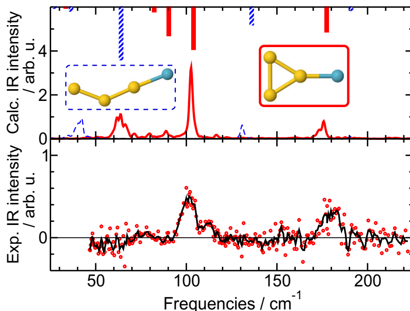
Figure 3. FIR-MPD spectrum (lower panel) of \text{Au}_3 \cdot \text{Kr} at 100 K and theoretical IR spectra (upper panel) at T = 100 K ( \bar{T} = 96 K) of the two isomers of \text{Au}_3 \cdot \text{Kr} . The harmonic spectra are plotted as bars upside-down. The horizontal line in the bottom panel marks the zero cross section. The dashed lines and bars refer to the obtuse-angled isomer, while the solid lines and bars refer to the acute-angled one.
