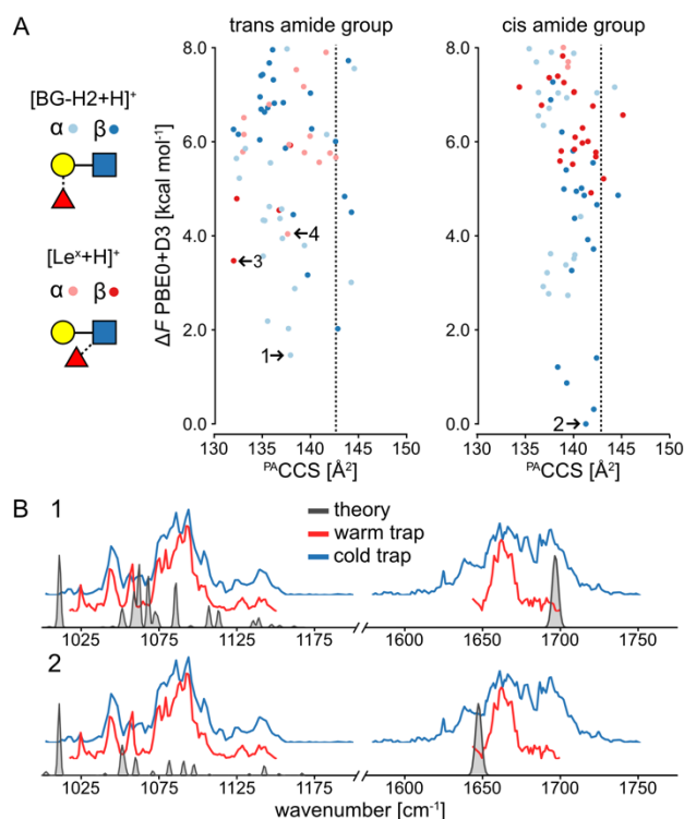
Figure 2. A) The {}^P\text{A} \text{CCS} vs relative free energy ( \Delta F ) of conformers of the [\text{Le}^x+\text{H}]^+ and [\text{BG}-\text{H}_2+\text{H}]^+ at PBE0+D3/6-311+G(d,p) level of theory. The dashed line indicates the experimental CCS, and the free energies are plotted relative to the lowest-free energy conformer of [\beta\text{-}c\text{-BG}-\text{H}_2+\text{H}]^+ . The most stable anomers of each ion are highlighted. B) The comparison of the experimental and vibrational spectrum of the most stable anomers of [\text{BG}-\text{H}_2+\text{H}]^+ . The comparison of the experimental and vibrational spectrum of the most stable anomers of [\text{Le}^x+\text{H}]^+ is shown in Figure S4.
